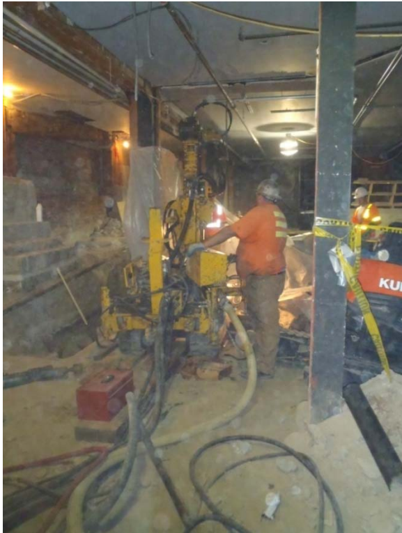
Drill Rig in Theater
