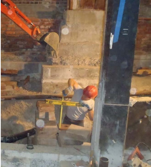
Economy Market Elevator Pit – Market Theater
